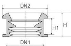
DN 110
