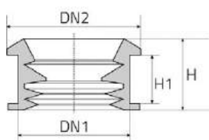
DN 110
