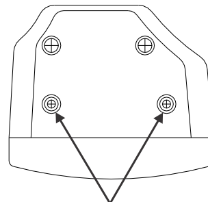
2 RIGGING POINTS M8 ON TOP AND BOTTOM
