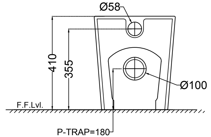
BACK VIEW
