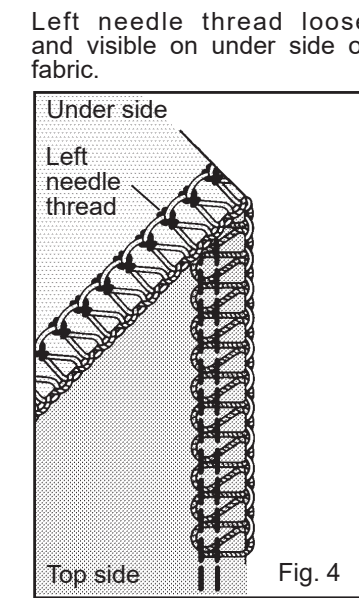
C: Left needle thread tighter Both looper looser
