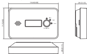
Image 3-1 Dimensions (mm[inch])
