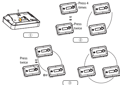
Figure 5-1 Interconnect device
