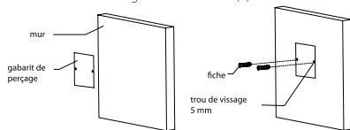
Image 7-4 Installation (1)
