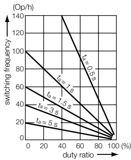
Intermittent periodic duty, t_a : Motor starting time
