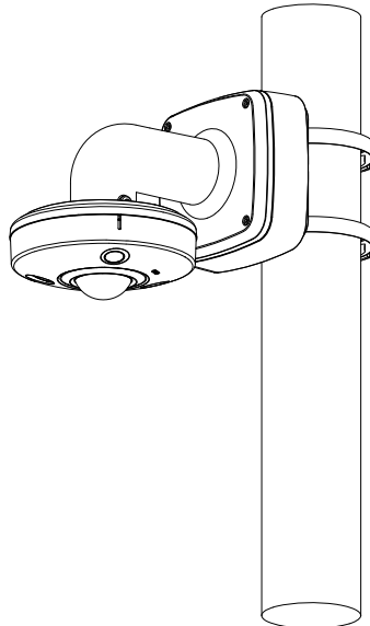
Pole Mount(Vertical)
