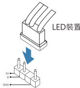
Addressable RGB LED裝置接頭 (5V_LED)
