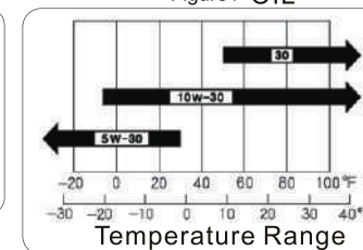
Figure2 OIL SAE GRADE
