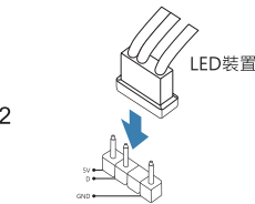
Addressable RGB LED裝置接頭 (5V_LED)
