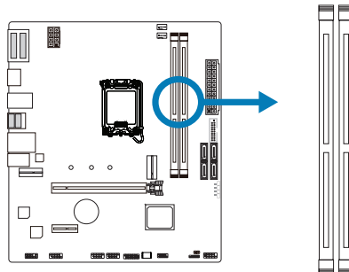
DDR4_A DDR4_B
