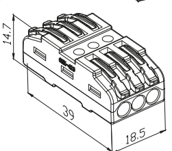
plc-smk-423
