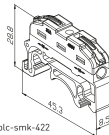
plc-smk-421-din
