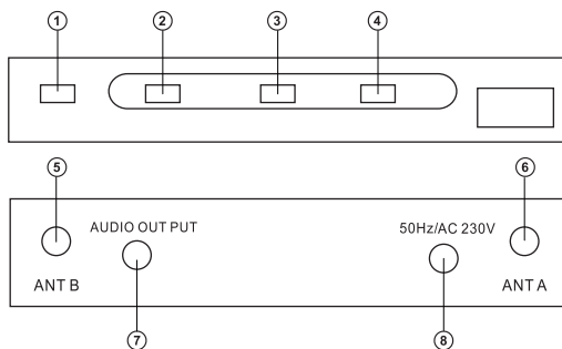
Fig. 1. Receiver
