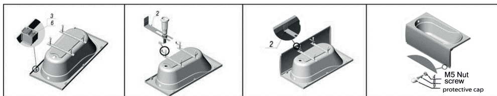
pic.3 - screen mount bracket installation
