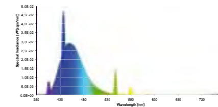
Colour spectrum actinic blue
