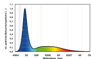
Colour spectrum powerLED+ marine hybrid
