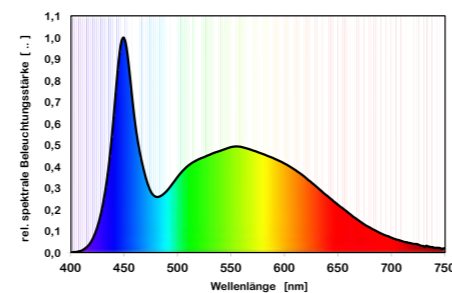
Colour spectrum powerLED daylight
