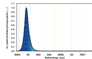
Colour spectrum powerLED+ marine actinic
