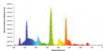
Colour spectrum daylight
