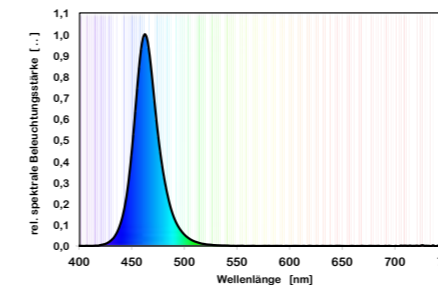
Colour spectrum powerLED actinic blue
