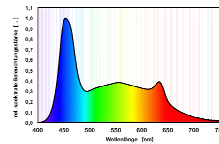
Colour spectrum powerLED plants
