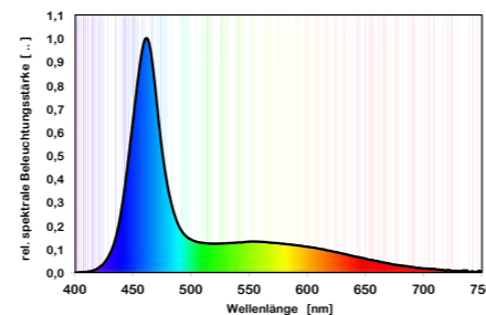
Colour spectrum powerLED hybrid
