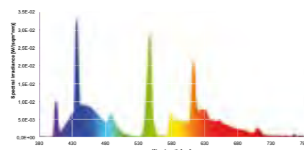
Colour spectrum plants
