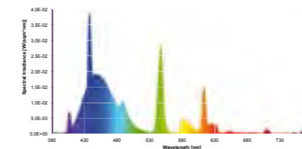
Colour spectrum hybrid
