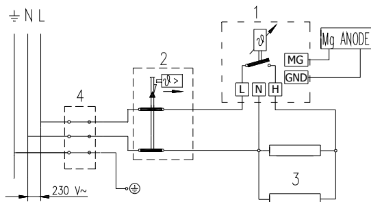
Electric installation
