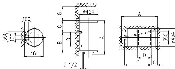
Connection and installation dimensions of the water heater [mm]
