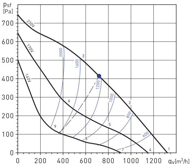
VENT /V-315N
