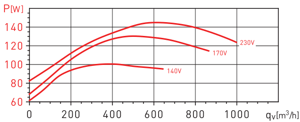
VENT /V-315N
