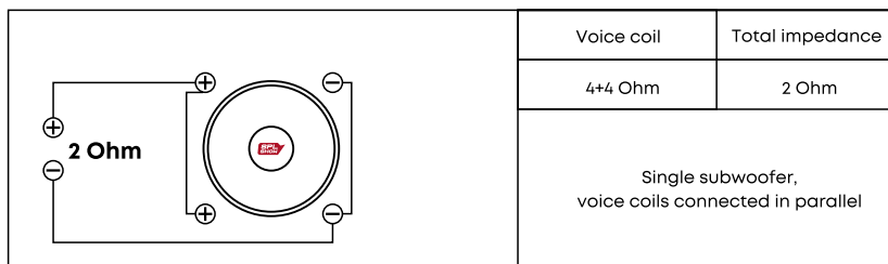
Connection diagram of subwoofer with dual VC 4+4 Ohm
