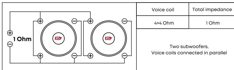
Connection diagram of 2 subwoofers with dual VC 4+4 Ohm
